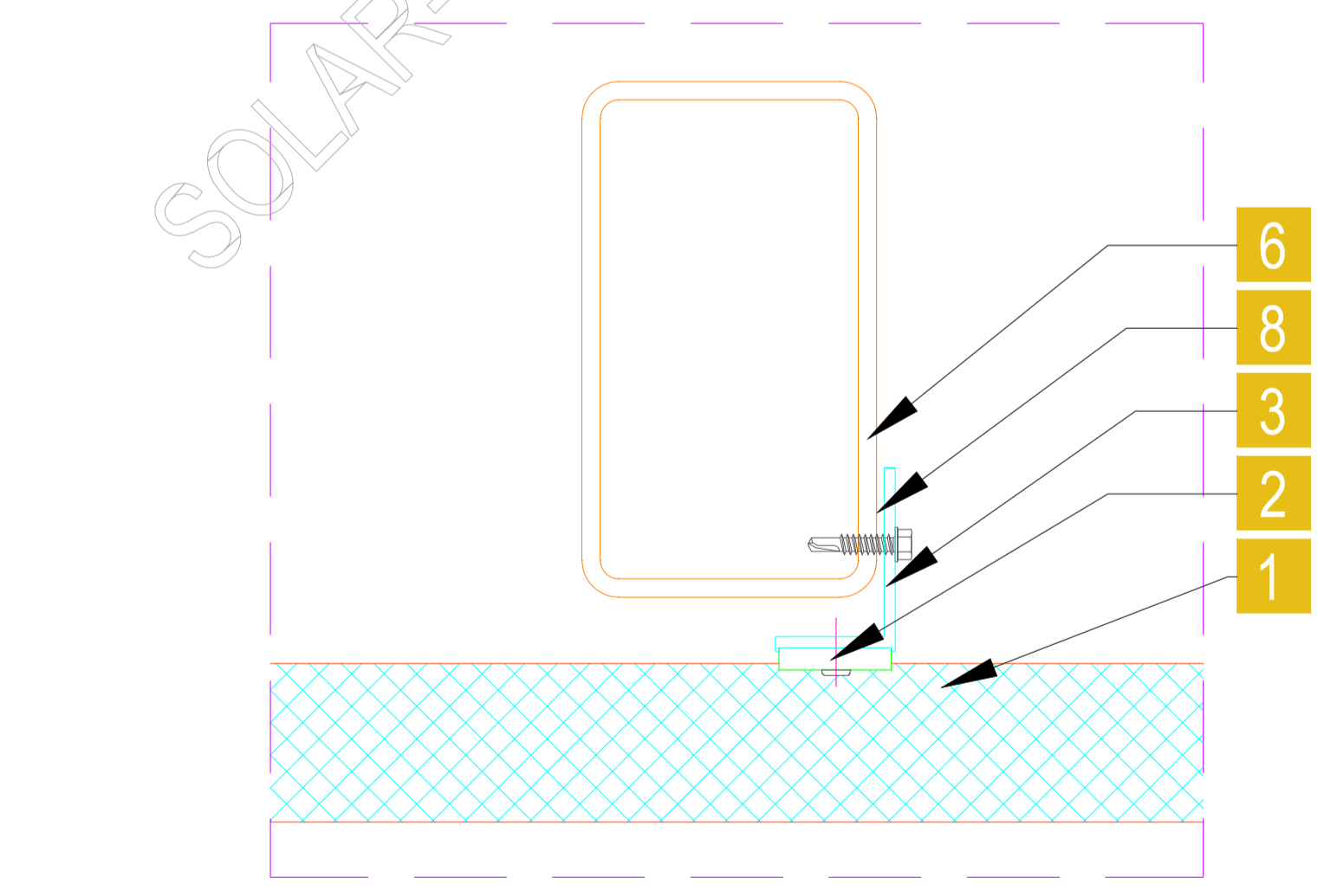
DETAIL 2 Option 3. Side connection.
