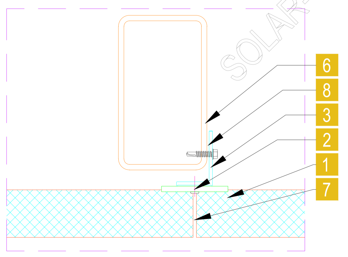
DETAIL 1. Side connection with dilatation.
